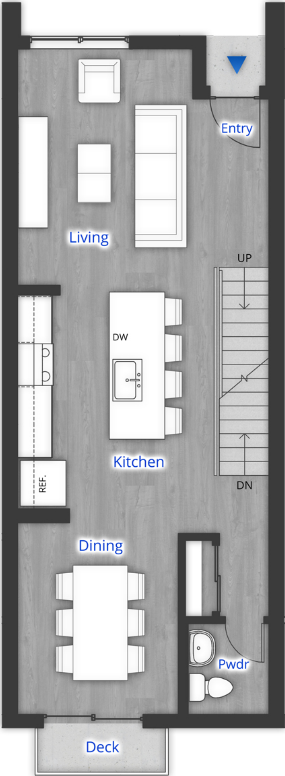
Main Level
